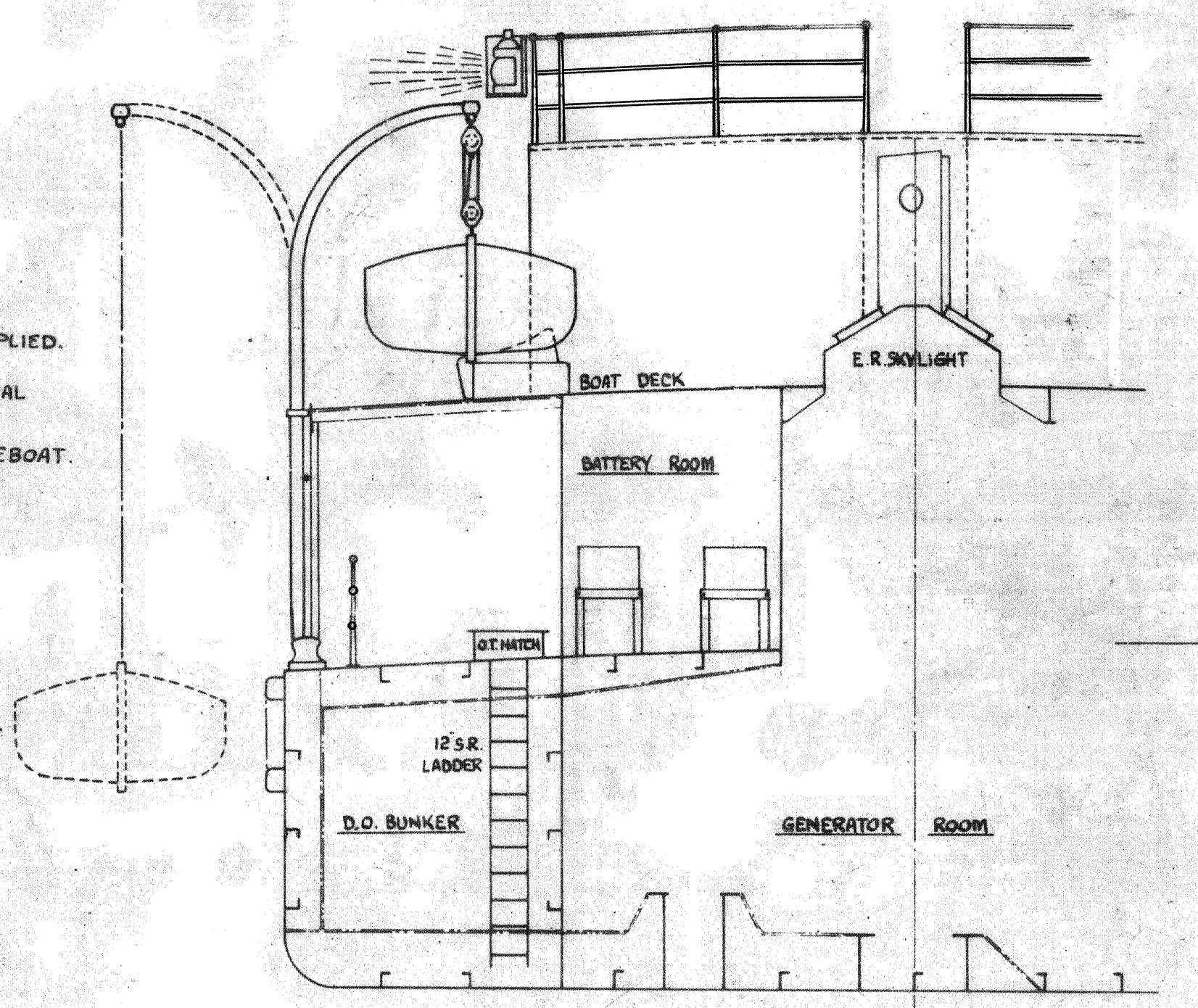
HALF SECTION AT LIFEBOAT DAVITS LOOKING AFT.
